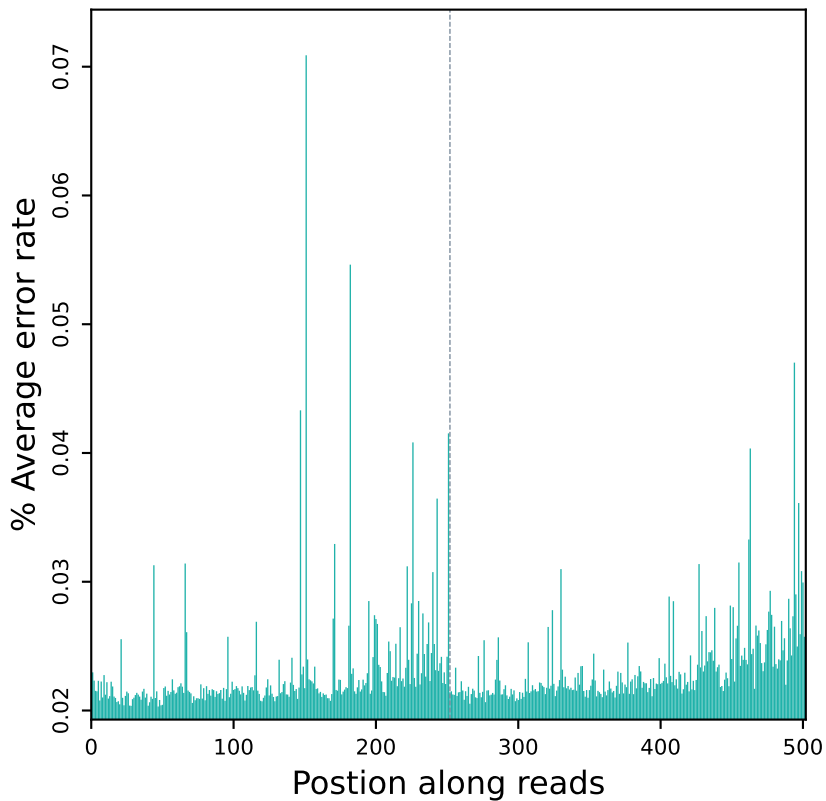
Error rate distribution along reads (R10719)
